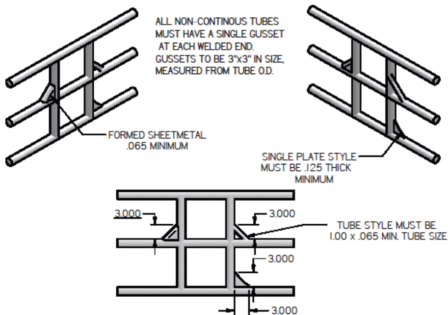
Figure 5 GUSSETS
